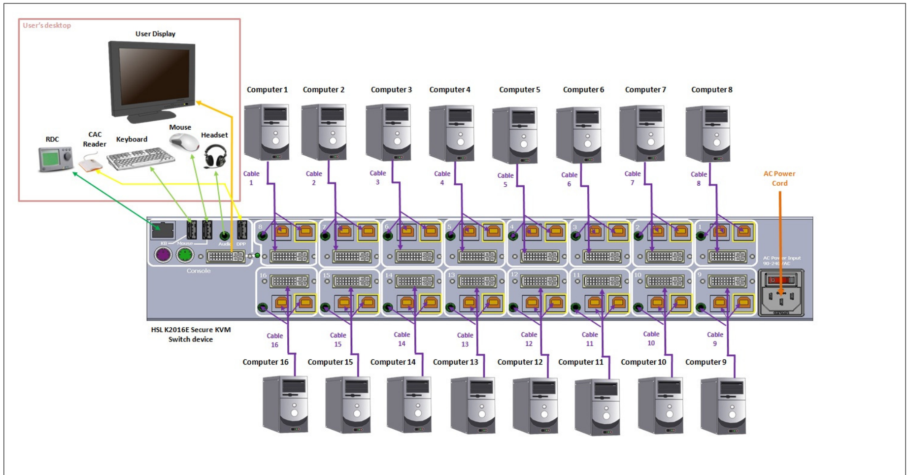
Typical system installation diagram (K2016E)
