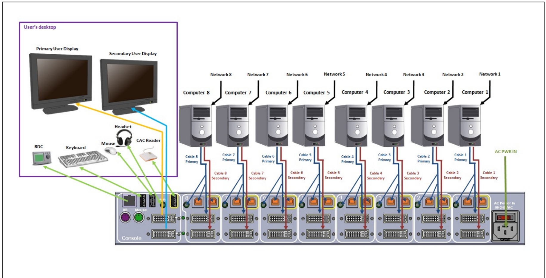
K248E typical system installation diagram
